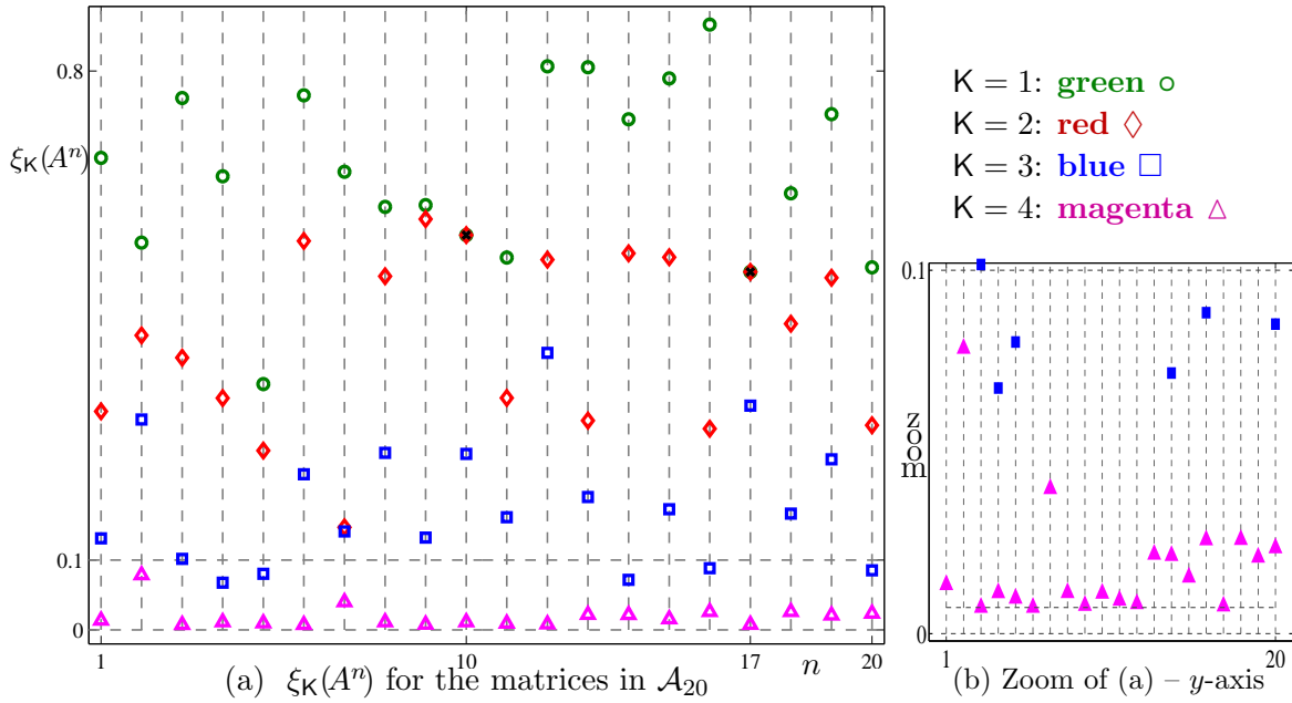
Figure 1. x -axis: the list of the 20 random matrices in \mathcal{A}_{20}^N . (a) y -axis: the value \xi_K(A^n) according to (58) for all K \in \mathbb{I}_{M-1} and for all n \in \mathbb{I}_{20} . The plot in (b) is a zoom of (a) along the y -axis.
