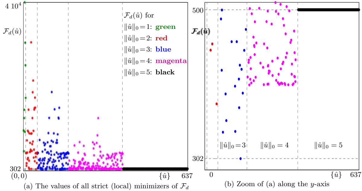
Figure 2. All 638 strict (local) minima of \mathcal{F}_d in (61) for \beta = 100 and data d corrupted with the arbitrary noise in (63). The x-axis lists all strict (local) minimizers \{\hat{u}\} of \mathcal{F}_d sorted according to their \ell_0 -norm \|\hat{u}\|_0 in increasing order. (a) The y-axis shows the value \mathcal{F}_d(\hat{u}) of these minimizers marked with a star. The value of \mathcal{F}_d for \hat{u} = 0 is not shown because it is too large ( \mathcal{F}_d(0) = 60559 = \|d\|^2 ). (b) A zoom of (a) along the y-axis. It clearly shows that \mathcal{F}_d has a very recognizable unique global minimizer
