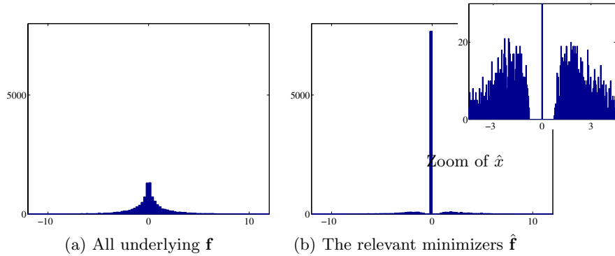
Figure 1. Histograms for 10 000 independent trials: \mathbf{f} and \hat{\mathbf{f}} for \varphi(t) = \sqrt{|t|} .
