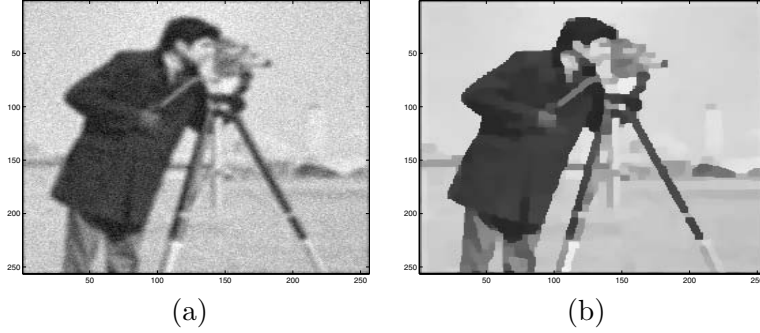
Figure 17. (a) Observed image; (b) the restored image.
