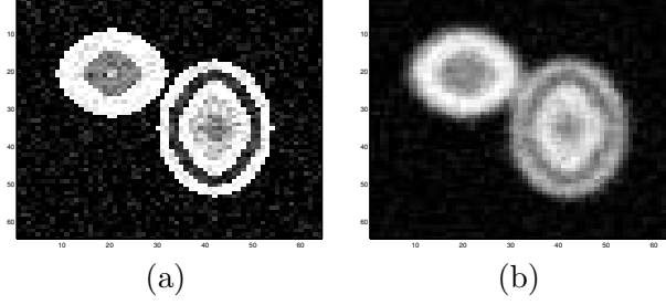
Figure 3. Observed circles images: (a) all pixels are contaminated by Gaussian noise with deviation 0.1 without blurring; (b) Gaussian blurring and all pixels are contaminated by Gaussian noise with deviation 0.05.
